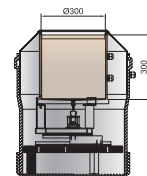
Ready-To-Go-Lysimeter Variations/Sizes
